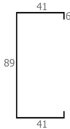
89mm x 41mm X 6mm LC PURLINS
