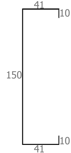
150mm x 41mm X 10mm LC PURLINS
